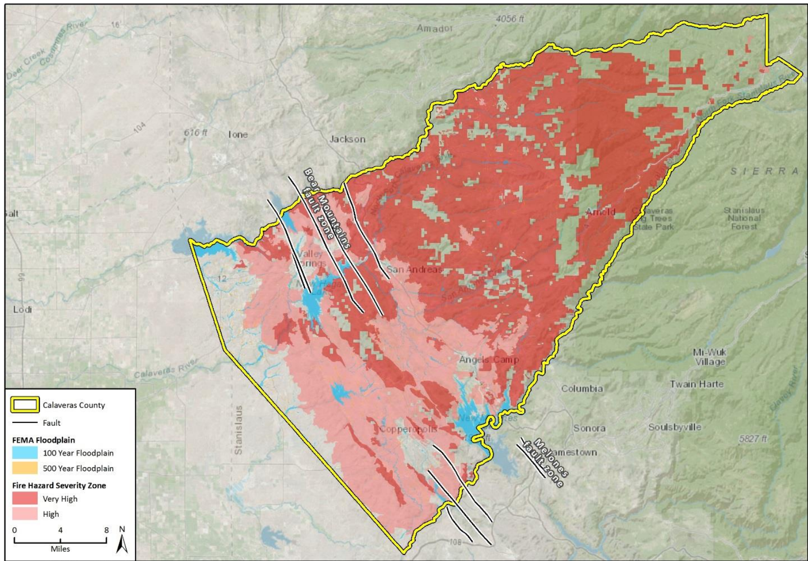
Fig 2 Natural Hazard Risks in Calaveras County
