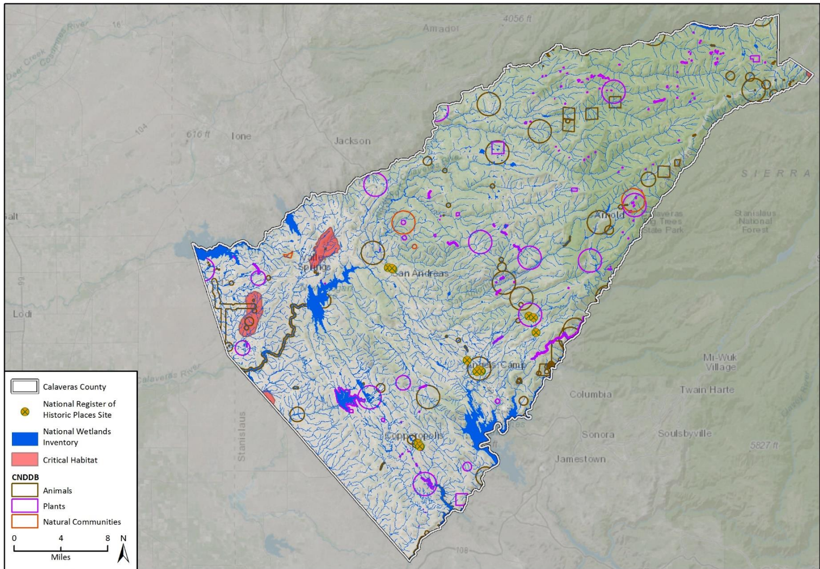
Fig 1 Resource Areas in Calaveras County
