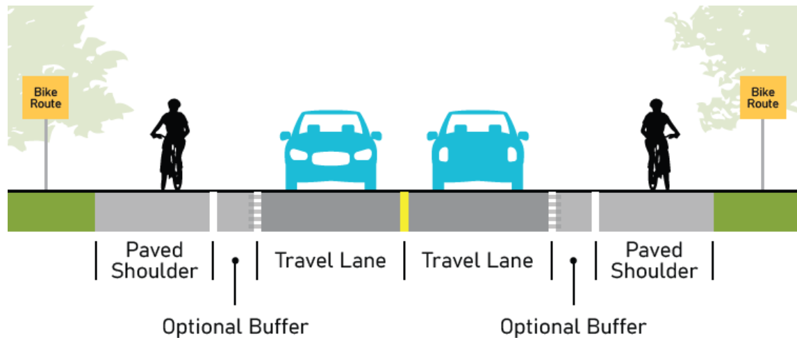
Figure 6: Paved Shoulder
