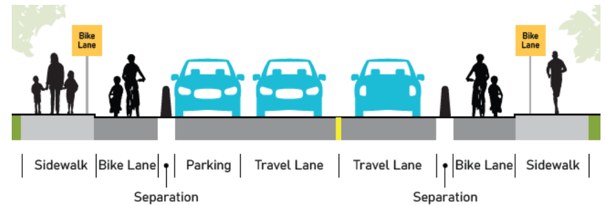
Figure 3: Separated Bikeway
